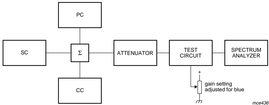
Fig 5. Test set-up intermodulation
